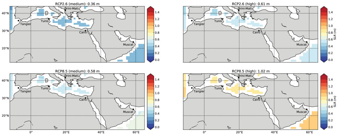
Figure 4.10: Patterns of regional sea-level rise (m).
